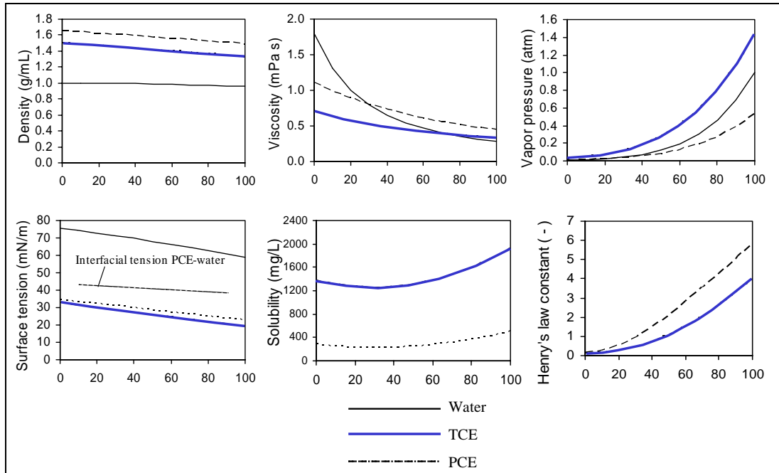
Figure 2. Properties of water, PCE and TCE as a function of temperature between 0 and 100°C. The x-axes represent degrees Celsius.
